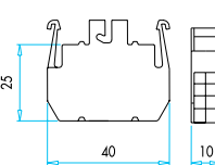
B Serisi Ampul Takılabilen Işıklı Blok Neon Lamp Mountable B Series Light Block
